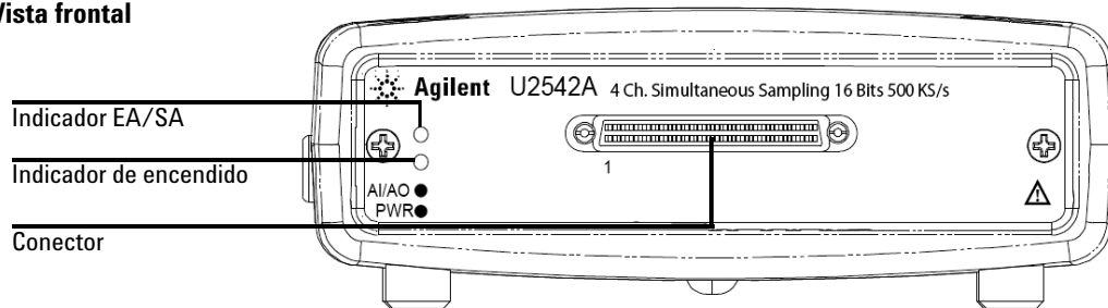
Vista frontal
